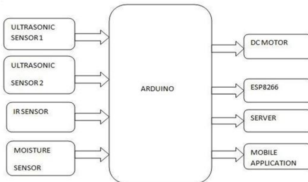
Figure: Schematic diagram of the smart waste management system
