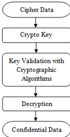
Figure 2: Usual Decryption
