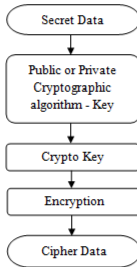
Figure 1: Usual Encryption
