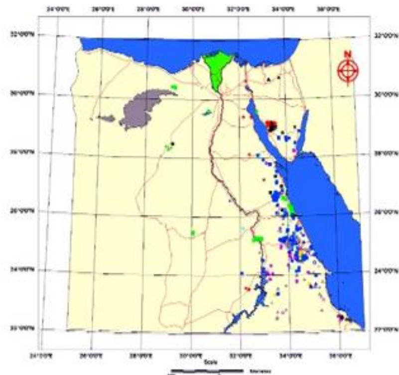
Fig. 7 Mineral Occurrence in Egypt
