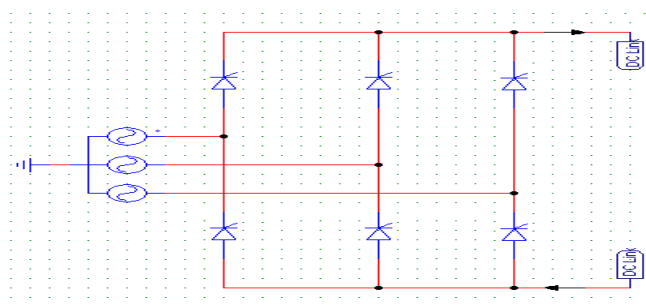
Figure:5 6- pulse LCC circuited. DC Cables
