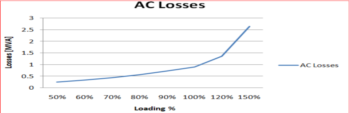
Figure 8: AC System Losses under different loading conditions
