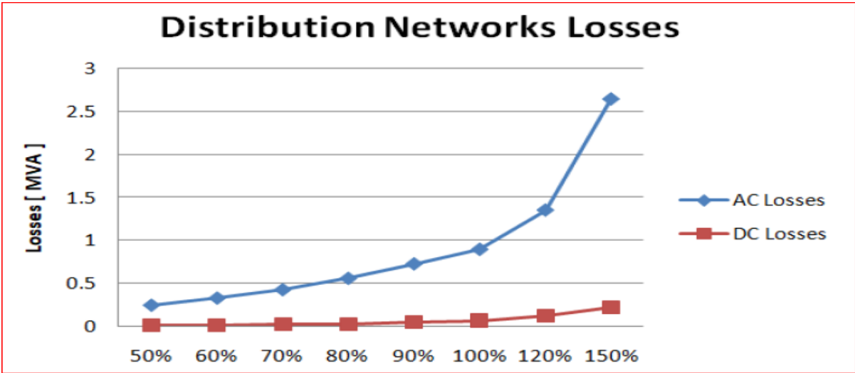
Figure 10 : AC & DC Systems Losses under different loading conditions.
