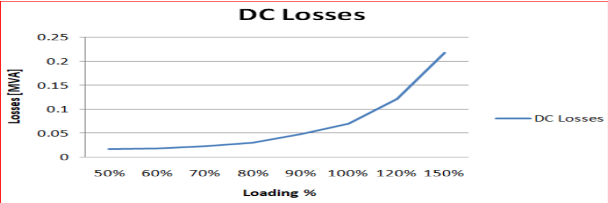
Figure 9: DC System Losses under different loading conditions
