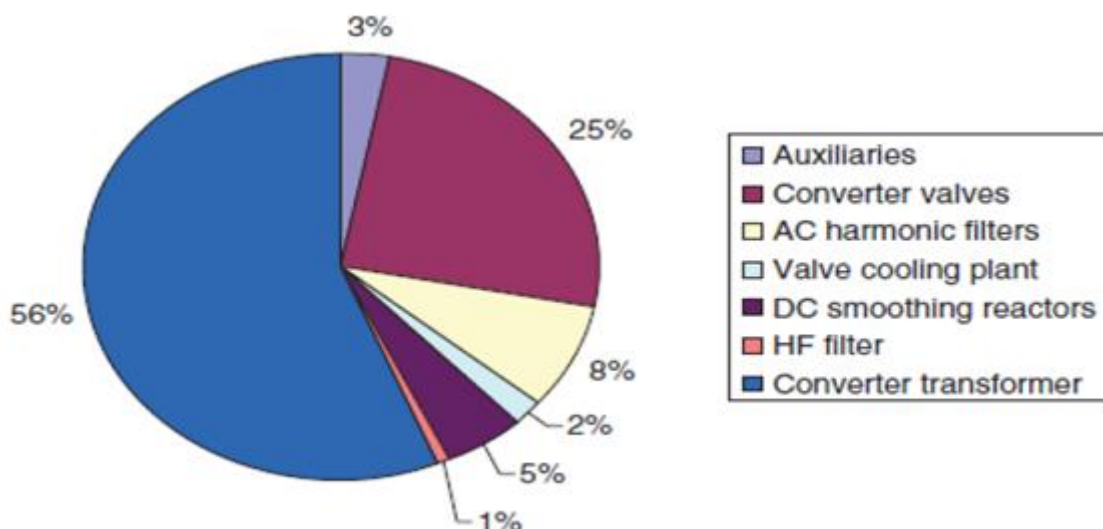
Figure: 2 break down LCC converter Station loss
