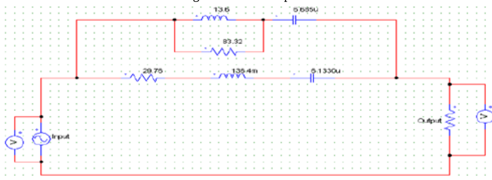
Figure: 6 High pass and RLC damped filter design
