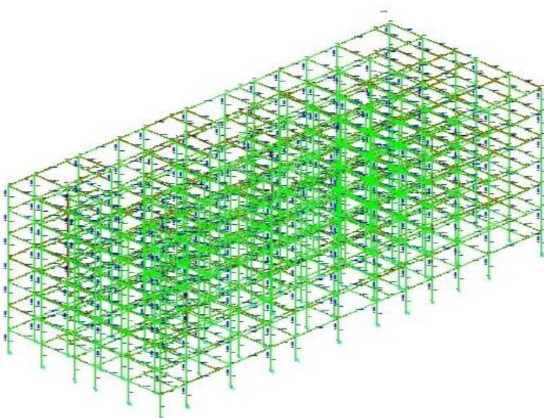
Fig 15 Deflection diagram
