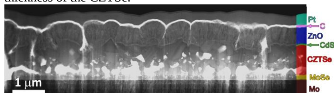
Figure 1: STEM bright field image of the cross section of a CZTSe solar cell. The white spots are voids in the CZTSe film while the top continuous white layer is the protective carbon coating.
