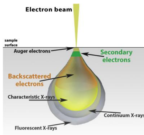
Fig. 3. Working principle of SEM. Sample characteristics from different sample depth can be detected by collecting different sources of information, such as secondary electrons, backscattered electrons, and characteristic X-rays. (Reprinted with permission from Nano Science Instrument) 47 .
