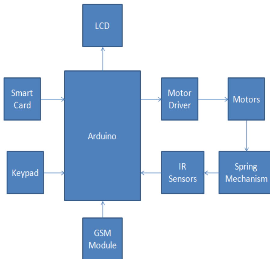
Fig 1 :block diagram
