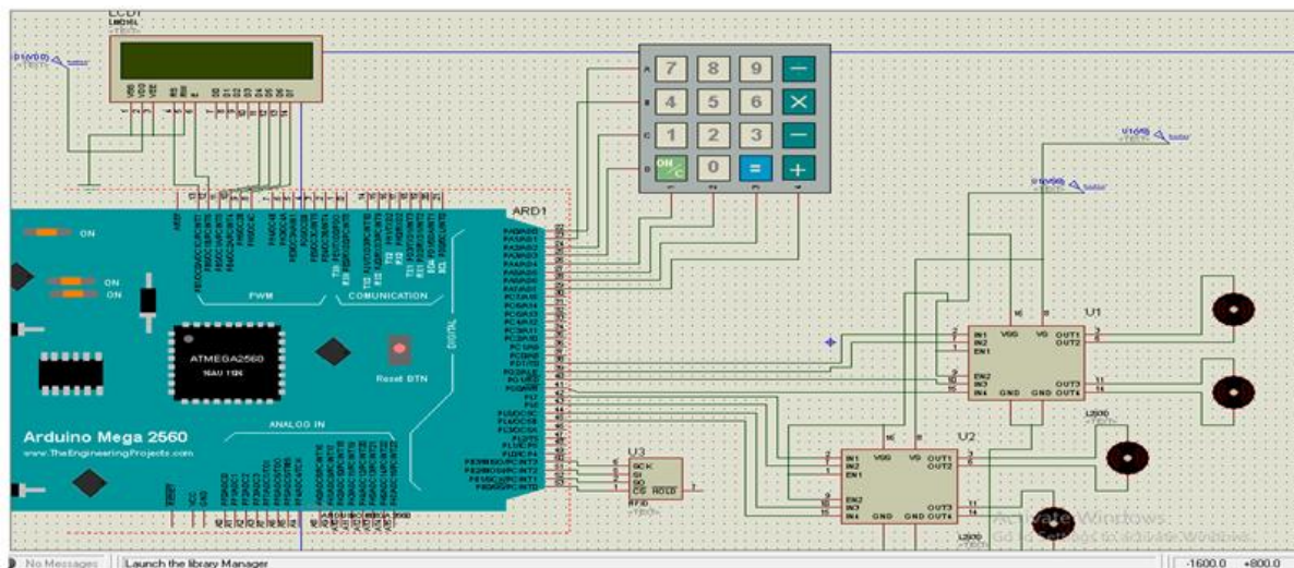
Fig 2 : circuit diagram of vending machine
