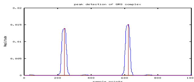
Figure XIV Peak Detection
