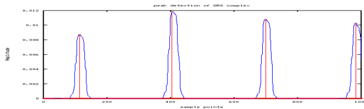
Figure VI Peak Detection
