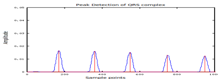
Figure X Peak detection
