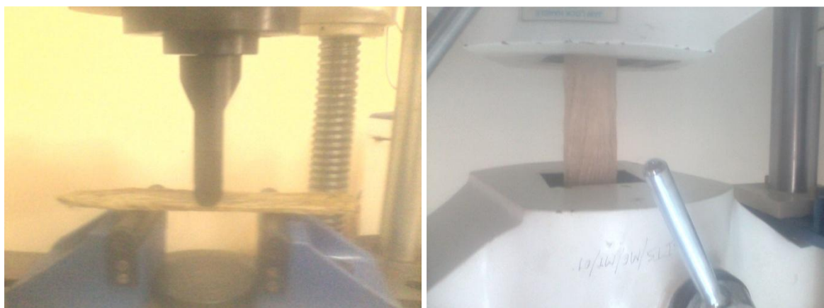
Figure 2.4 Composite Sample weighing & Mechanical Testing
