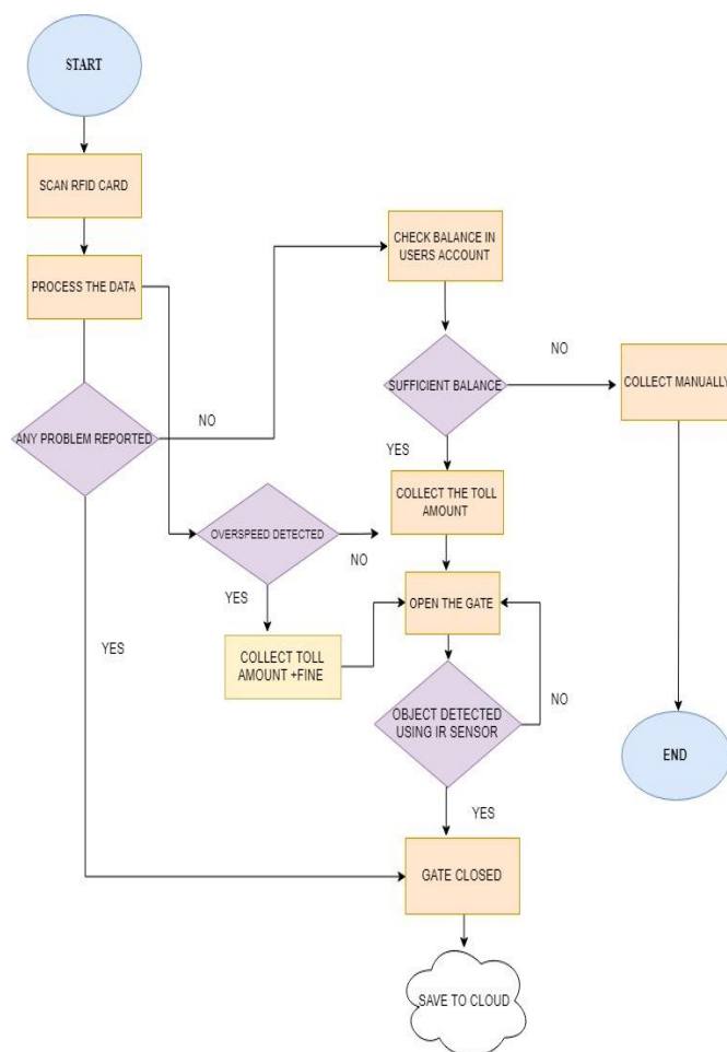
Fig 2. Flow Diagram
