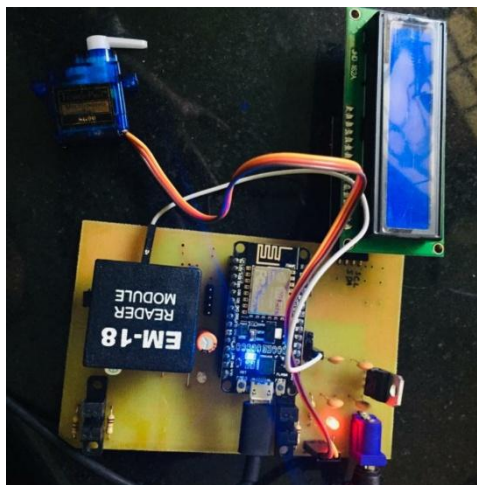
Fig.7 Hardware
