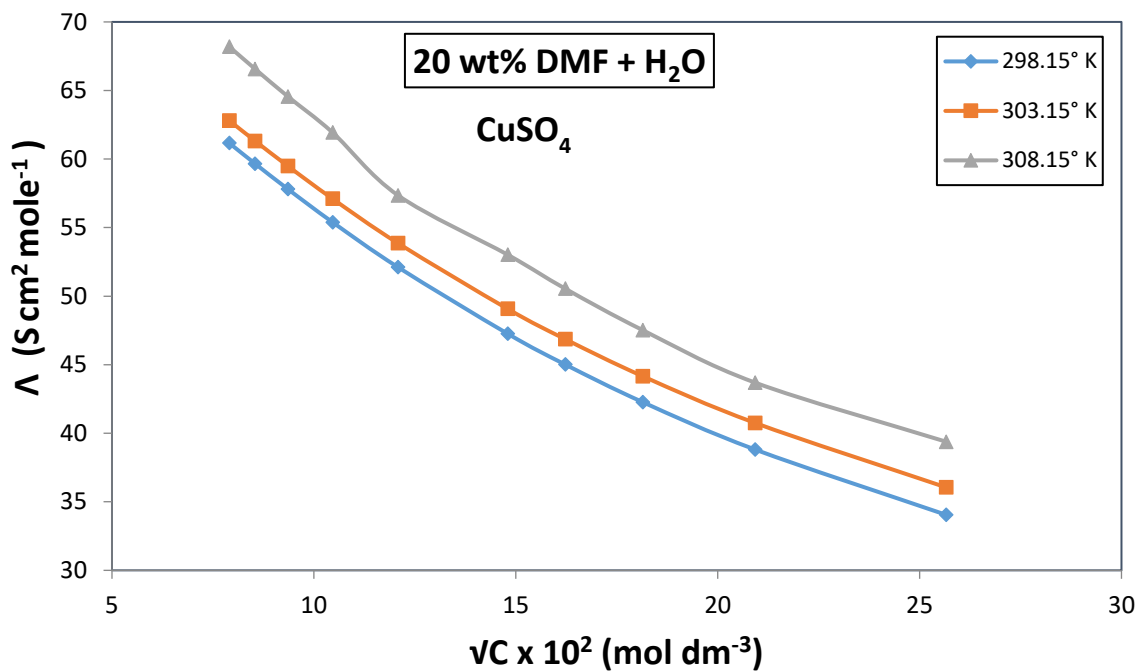
Fig. I B (2.5):-Plot of \Lambda vs. \sqrt{C} for CuSO 4 in DMF-H 2 O Mixture
