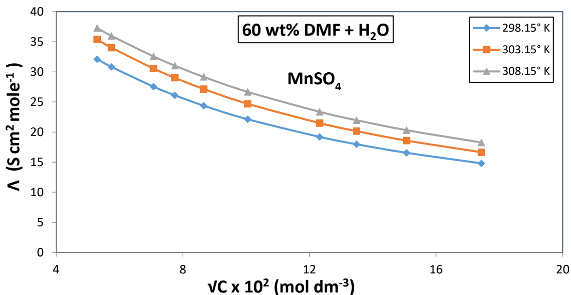
Fig. I B (2.13):-Plot of \Lambda vs. \sqrt{C} for \text{MnSO}_4 in DMF- \text{H}_2\text{O} Mixture
