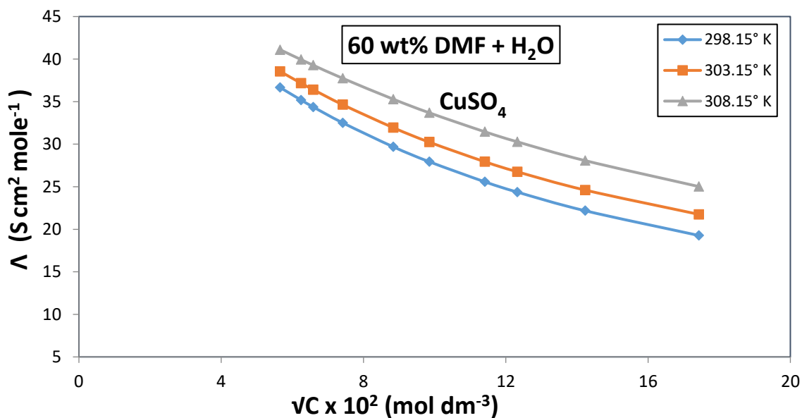
Fig. I B (2.14):-Plot of \Lambda vs. \sqrt{C} for \text{CuSO}_4 in DMF- \text{H}_2\text{O} Mixture
