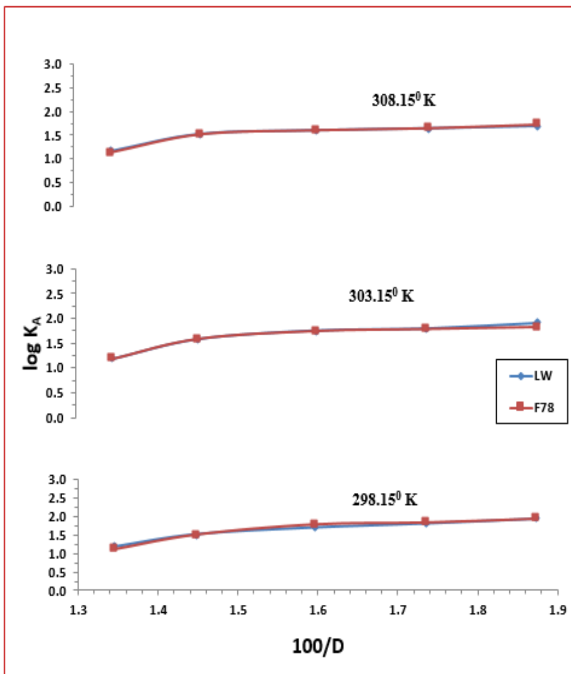
Fig. II B (3.3):-Plots of \log K_A vs 1/D for ZnSO 4 in DMF -H 2 O Mixtures at 298.15 ,303.15,308.15°K
