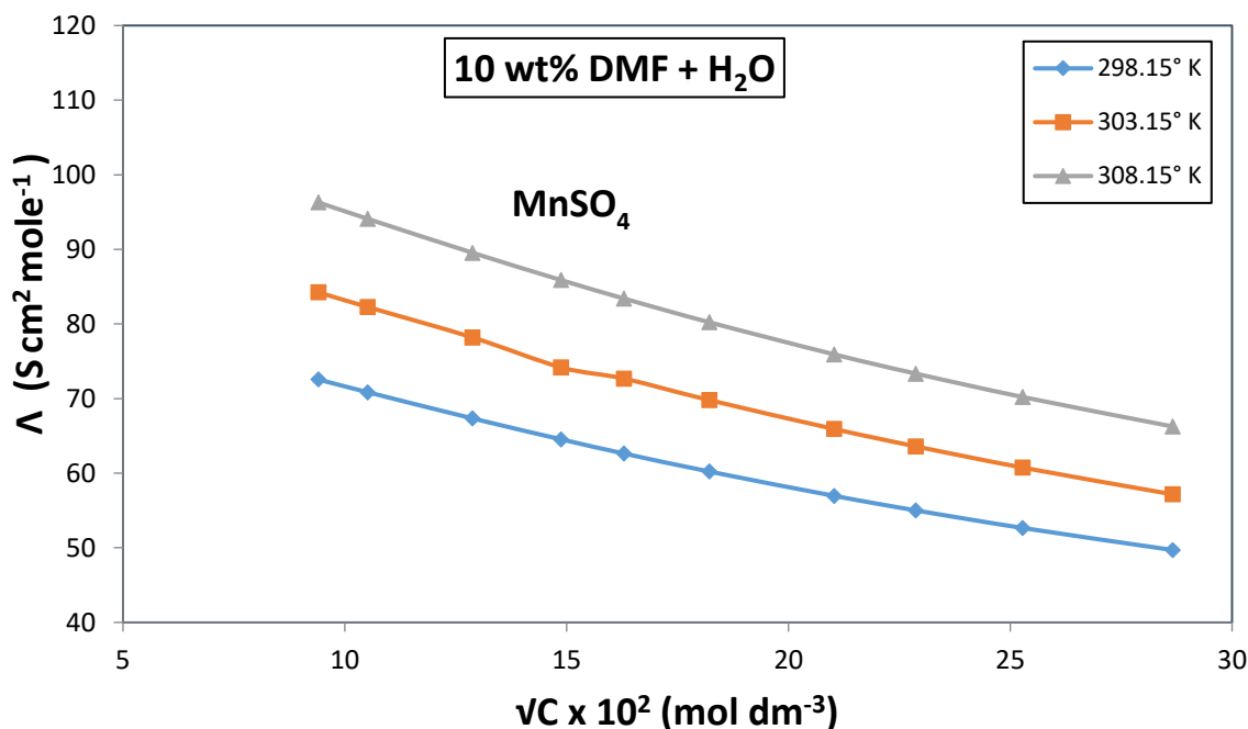
Fig. I B (2.1):-Plot of \Lambda vs \sqrt{C} for MnSO 4 in DMF-H 2 O Mixture
