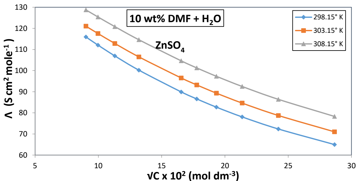
Fig. I B (2.3):-Plot of \Lambda vs. \sqrt{C} for ZnSO 4 in DMF-H 2 O Mixture
