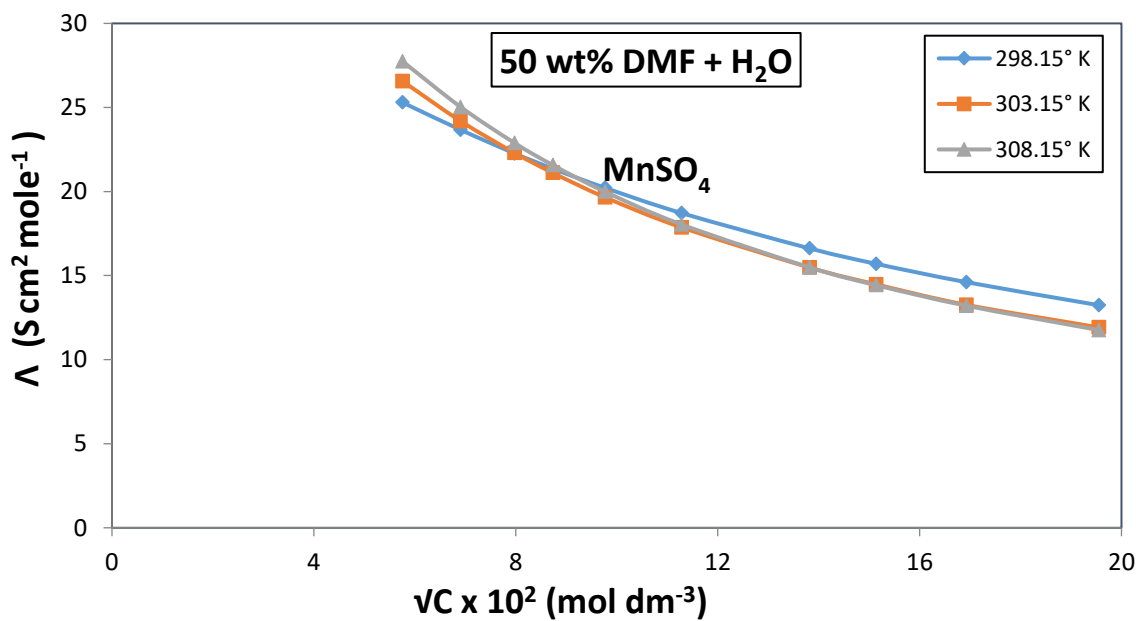
Fig. I B (2.10):-Plot of \Lambda vs. \sqrt{C} for MnSO 4 in DMF-H 2 O Mixture
