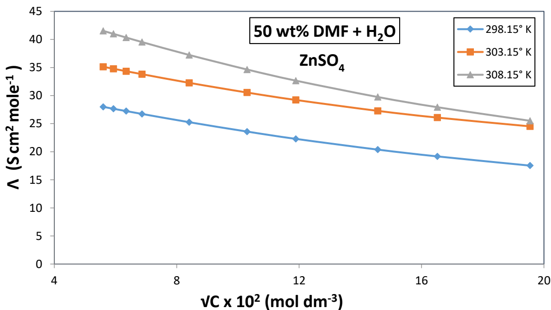
Fig. I B (2.12):-Plot of \Lambda vs. \sqrt{C} for ZnSO 4 in DMF-H 2 O Mixture
