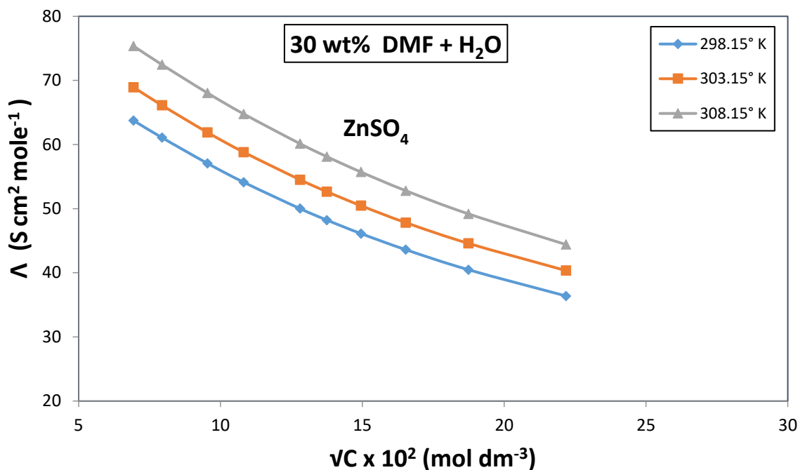
Fig. I B (2.9):-Plot of \Lambda vs. \sqrt{C} for ZnSO 4 in DMF-H 2 O Mixture
