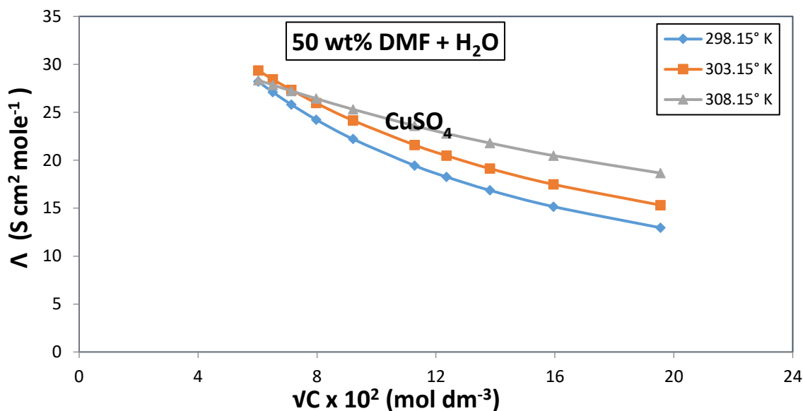
Fig. I B (2.11):-Plot of \Lambda vs. \sqrt{C} for CuSO 4 in DMF-H 2 O Mixture
