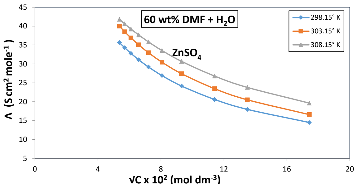
Fig. 1 B (2.15):-Plot of \Lambda vs. \sqrt{C} for \text{ZnSO}_4 in DMF- \text{H}_2\text{O} Mixture
