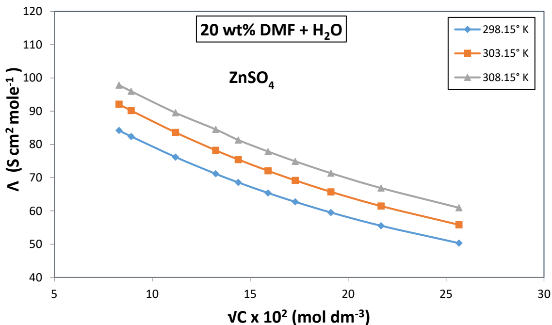
Fig. I B (2.6):-Plot of \Lambda vs. \sqrt{C} for ZnSO 4 in DMF-H 2 O Mixture
