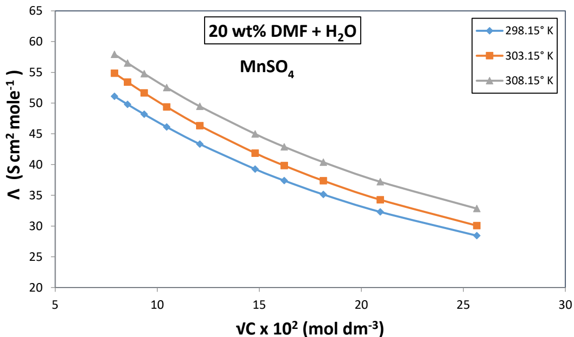
Fig. I B (2.4):-Plot of \Lambda vs. \sqrt{C} for MnSO 4 in DMF-H 2 O Mixture
