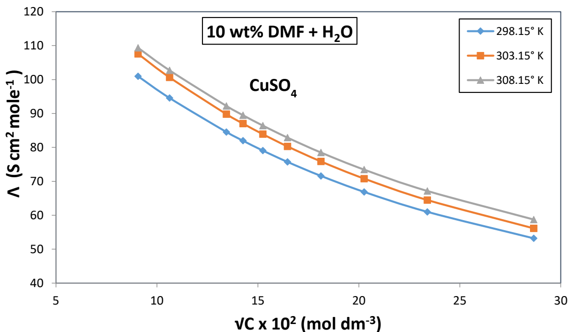
Fig. I B (2.2):-Plot of \Lambda vs \sqrt{C} for CuSO 4 in DMF-H 2 O Mixture
