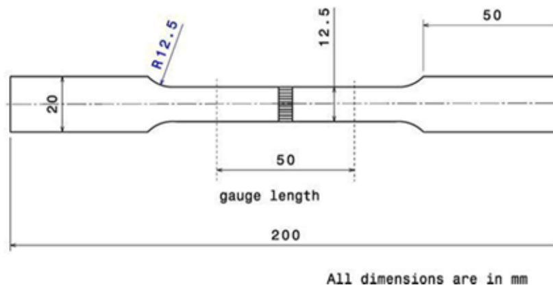
Figure: 3.3.2.1 Test Specimen
