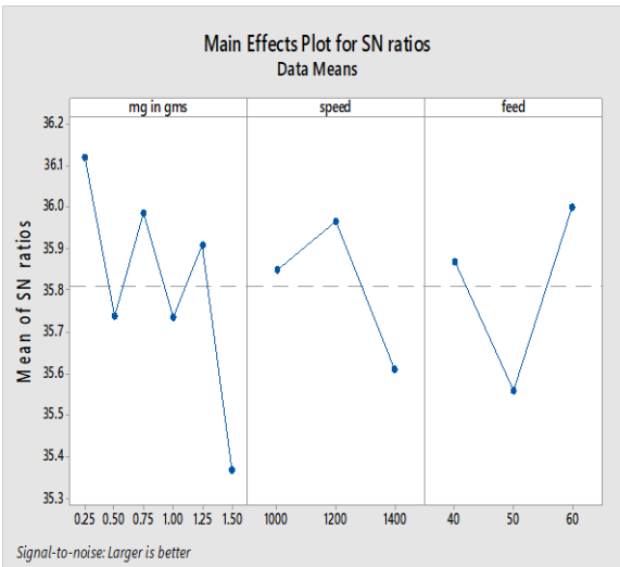
Graph: 4.2 S/N ratios for Hardness of AA 6061
