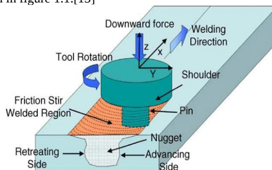
Fig. 1.1: Schematic representation of FSW process Table 1.1: Chemical composition of AA6061 in weight %.
