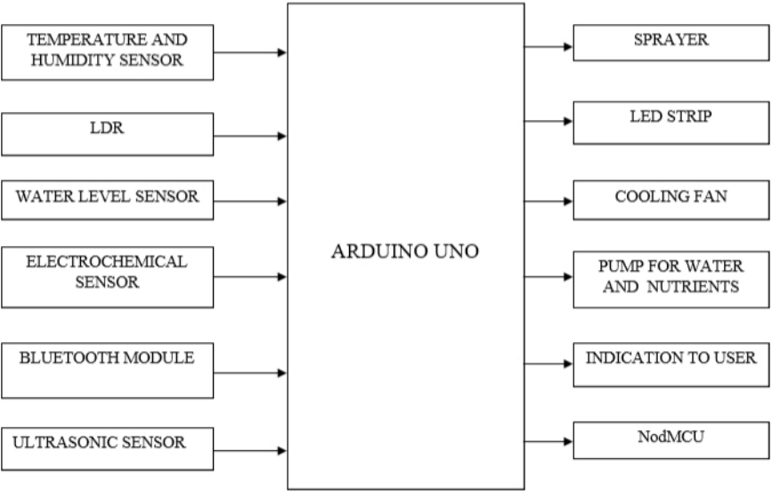
Figure 2.1. Block diagram for hydroponics system
