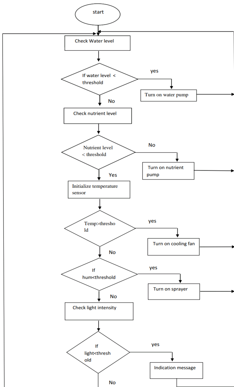
Figure 2.3 Flowchart for hydroponic system
