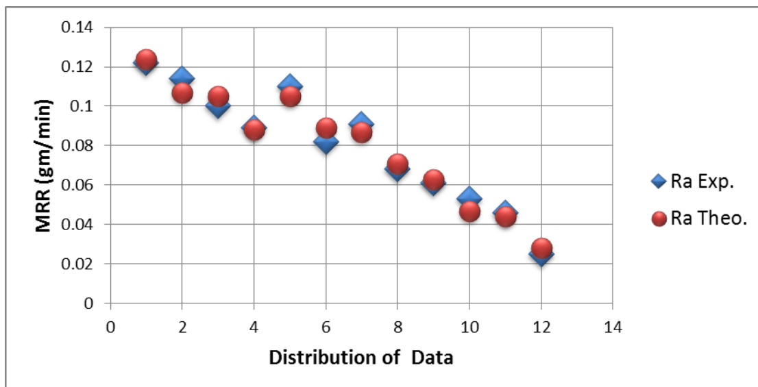
Figure (7) Comparison between Experimental and Theoretical MRR Data for SiC- Fe abrasive brush
