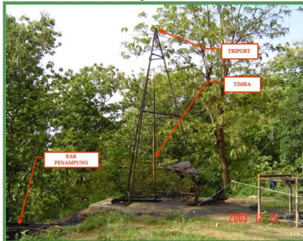
Figure 1. The Old Well Traditional Production Technology in the Banyubang field
