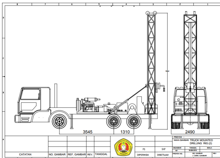
Figure 9. Design of Mobile Rig Technology Model
