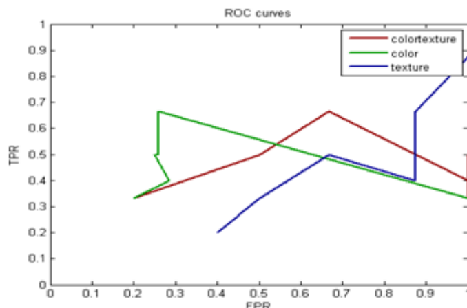
Figure 4.1 ROC curve
