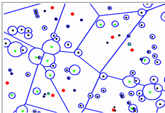
Figure 1.3: Layout of a PPP-based 3-tier HetNet of macrocells (large circles), picocells (triangle shpwng s) and femtocells (squares) where P_b = 100P_s = 1000P_f and \lambda_b = 4\lambda_s = 8\lambda_f
