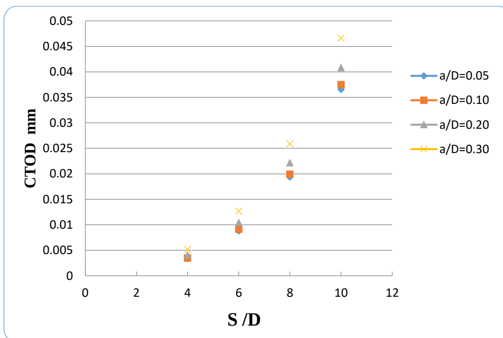
Fig.6. Variation of the CTOD according to S/D
